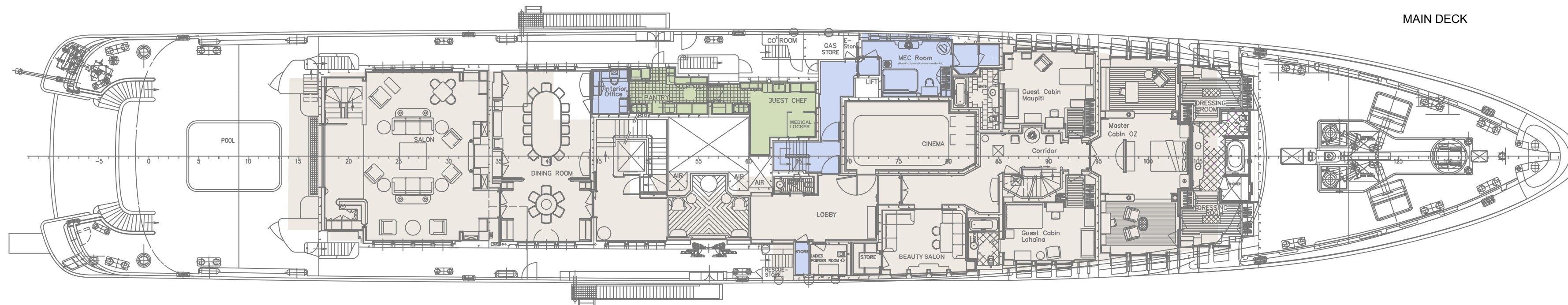
MAIN DECK
